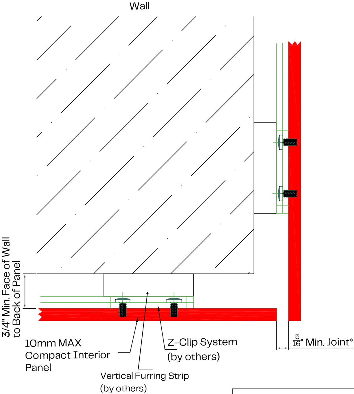
Max Compact Interior Z-Clip System Details Detail 5: Outside Corner
