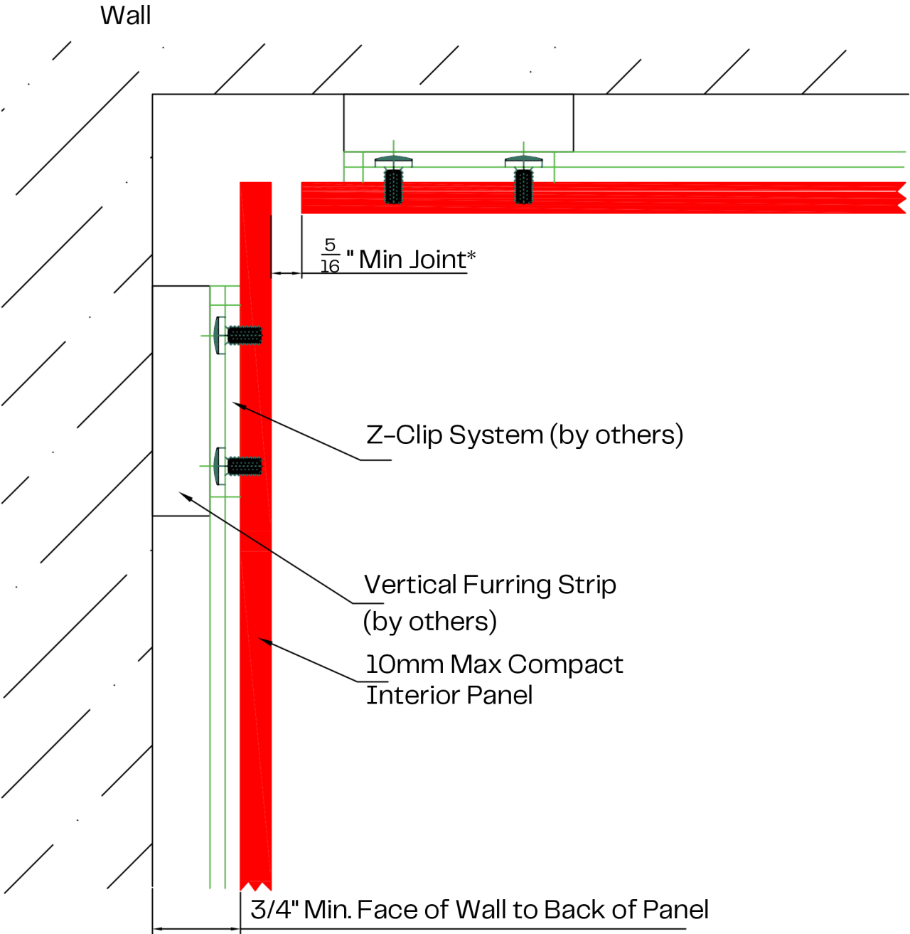
Max Compact Interior Z-Clip System Details Detail 4: Inside Corner
