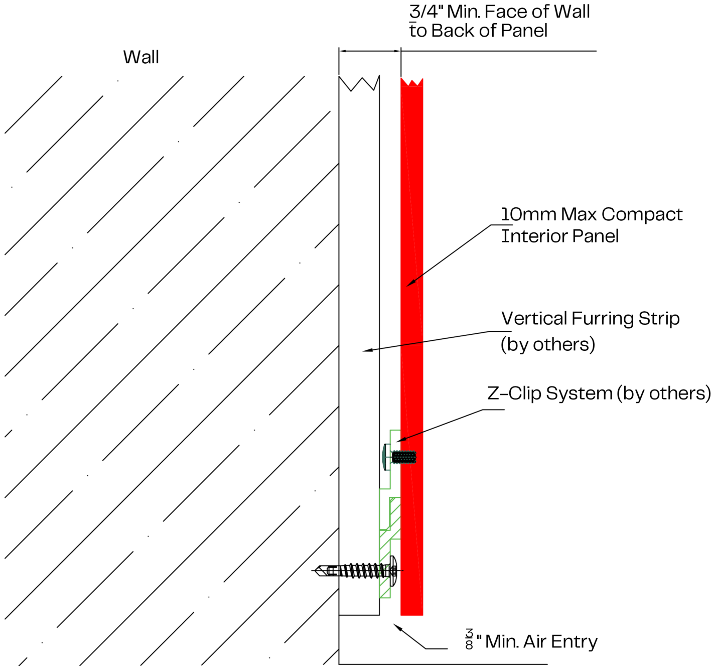
Max Compact Interior Z-Clip System Details Detail 3: Base of Wall
