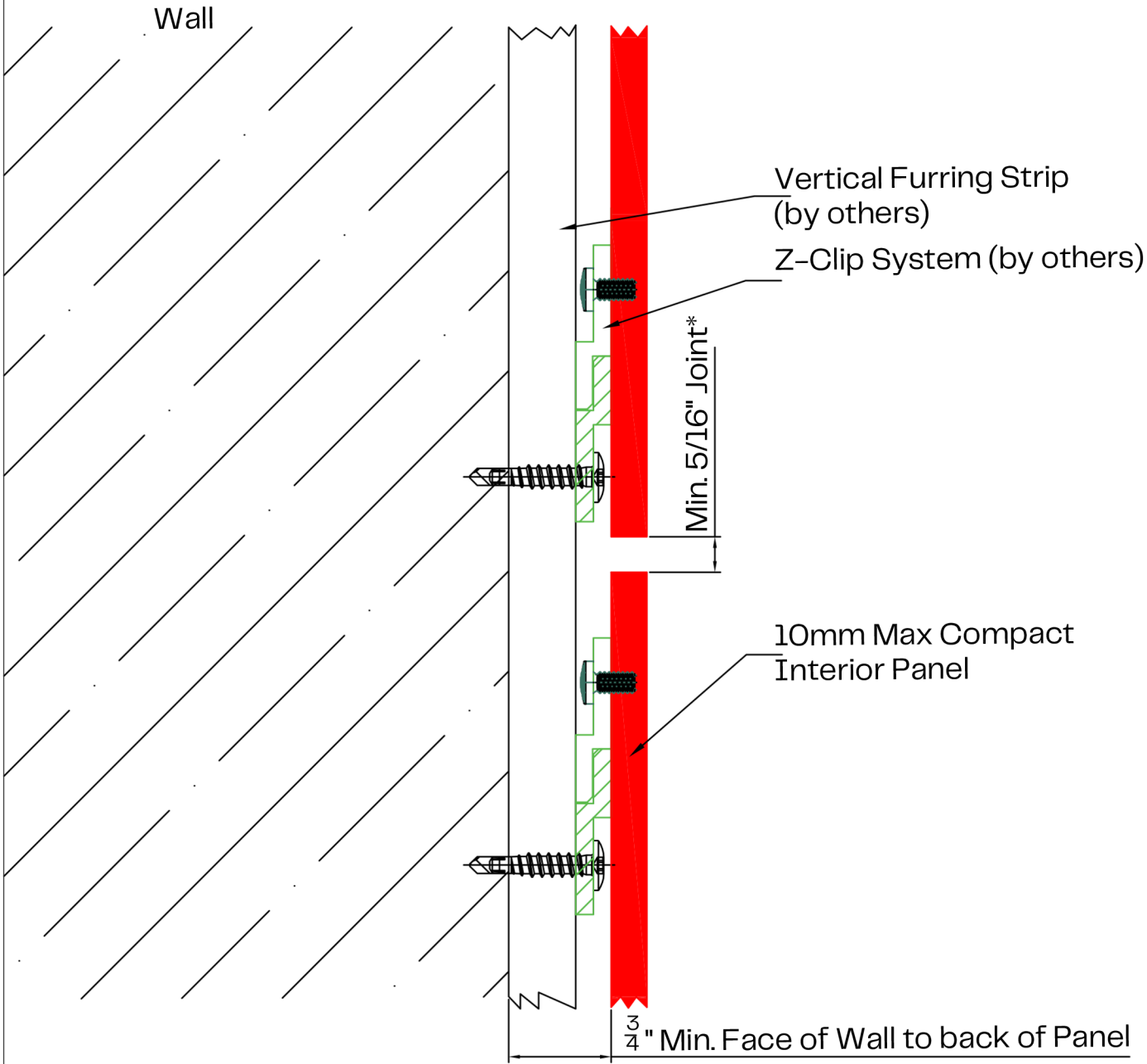
Max Compact Interior Z-Clip System Details Detail 2: Horizontal Joint
