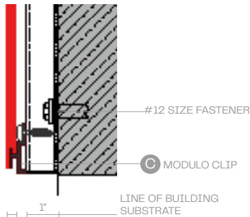
WINDOW LINTEL A101
