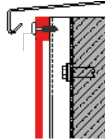
WINDOW SILL CONNECTION A102
