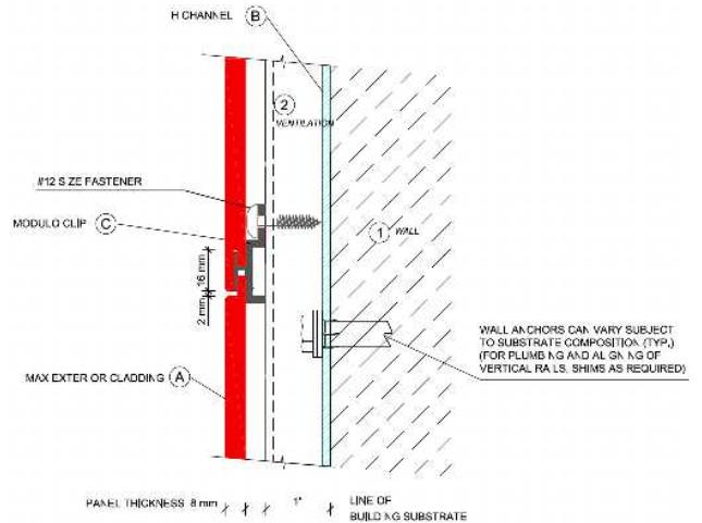
HORIZONTAL JOINT A110
