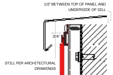
WINDOW SILL CONNECTION A102
