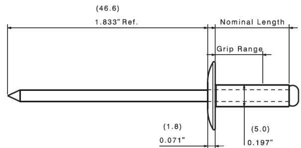
SFS AP16-5 Rivet for metal substructure
