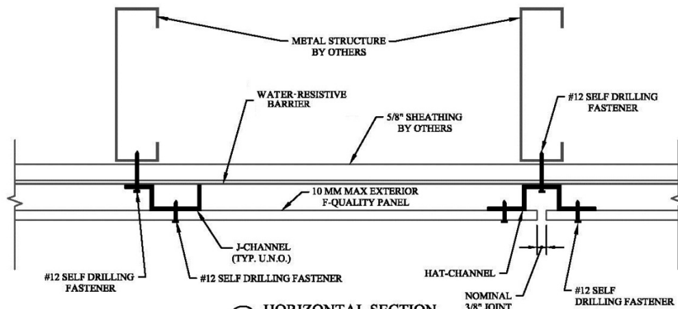
① HORIZONTAL SECTION INSTALLATION DETAILS
