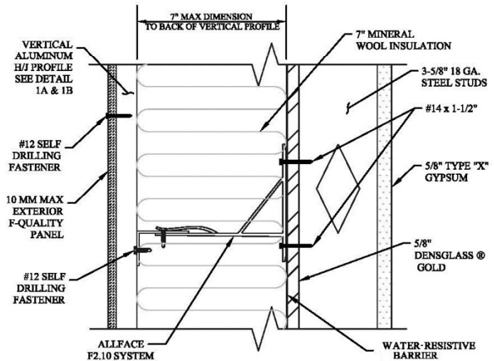
④ MAXIMUM INSULATION CAVITY DEPTH
