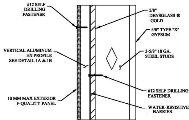
② VERTICAL EXTRUSION INSTALLATION
