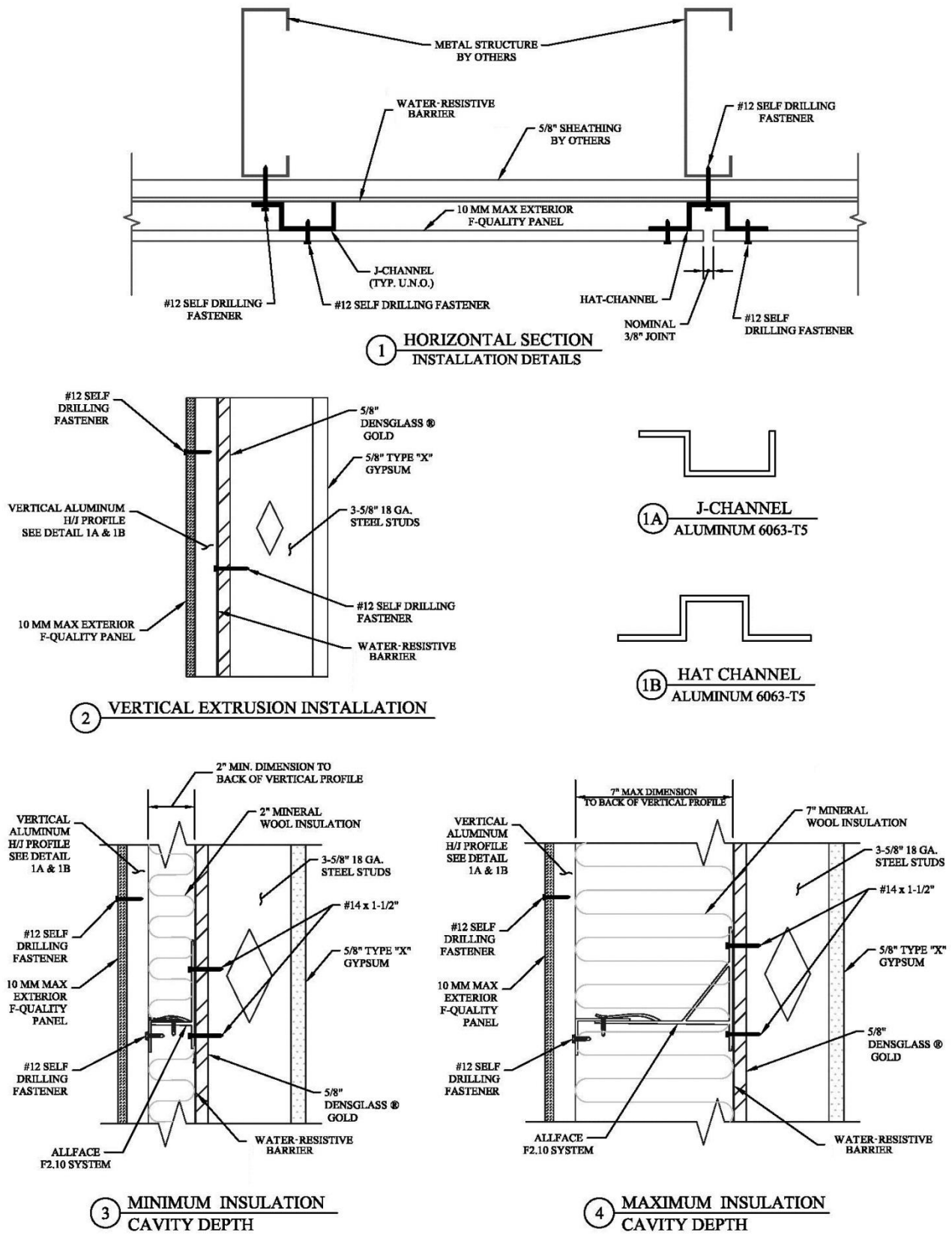
FIGURE 1—MAX COMPACT EXTERIOR F-QUALITY WALL PANEL CLADDING SYSTEM DETAILS
