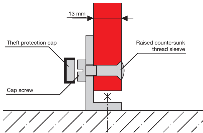
HORIZONTAL CUT FLOOR CONNECTION WITH AN L-PROFILE
