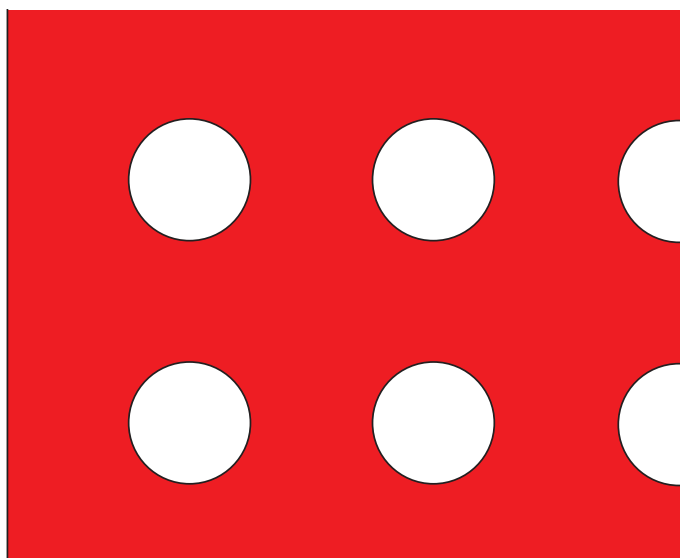
MINIMUM DISTANCES BETWEEN PERFORATIONS WITH FALL PROTECTION
